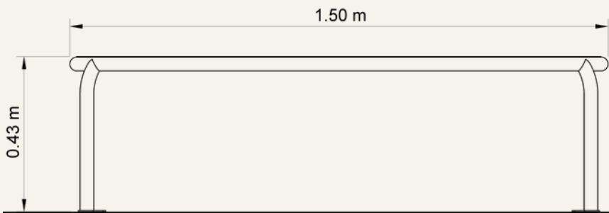
VISTA FRONTAL
